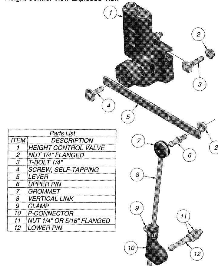
FIGURE 3 Height Control View Exploded View
